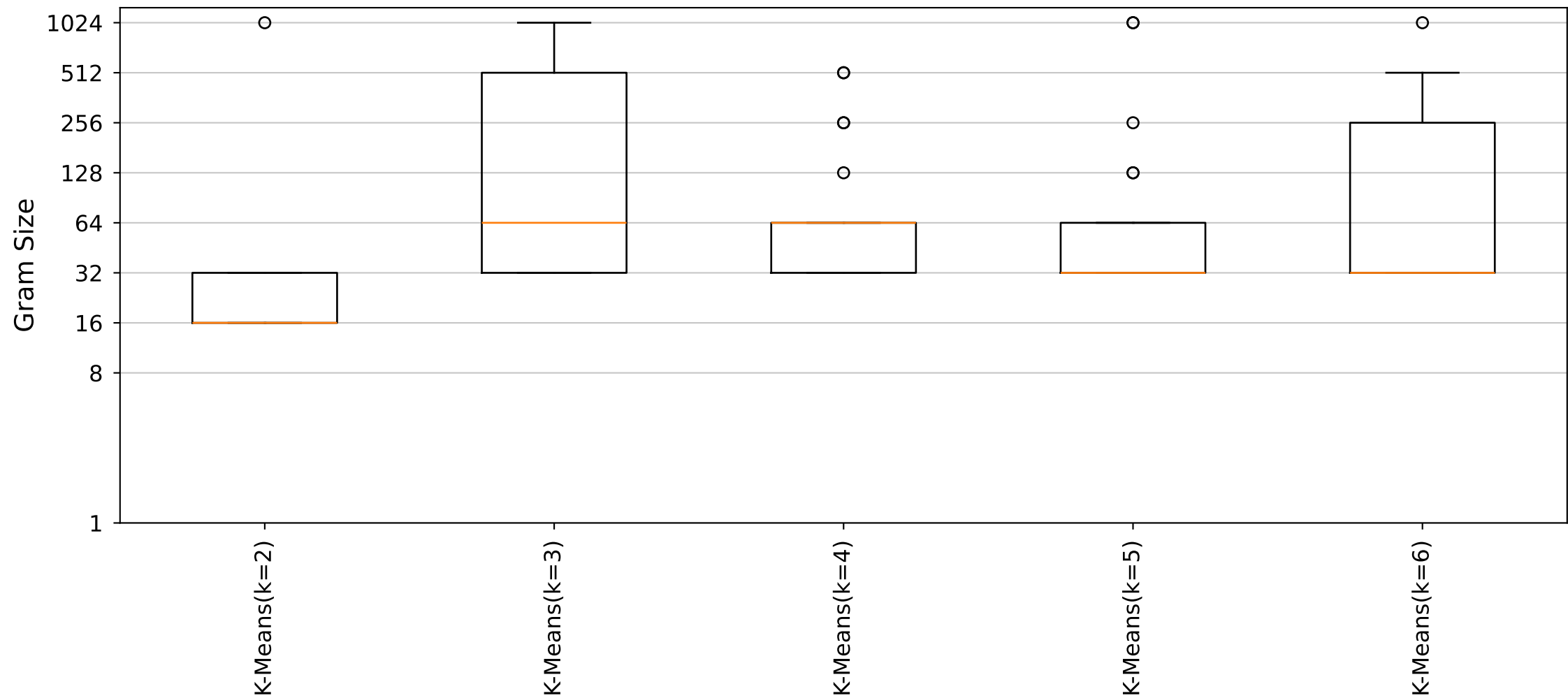
YARA Rules Gram Size Distribution (Cluster26_Size6 dataset)
